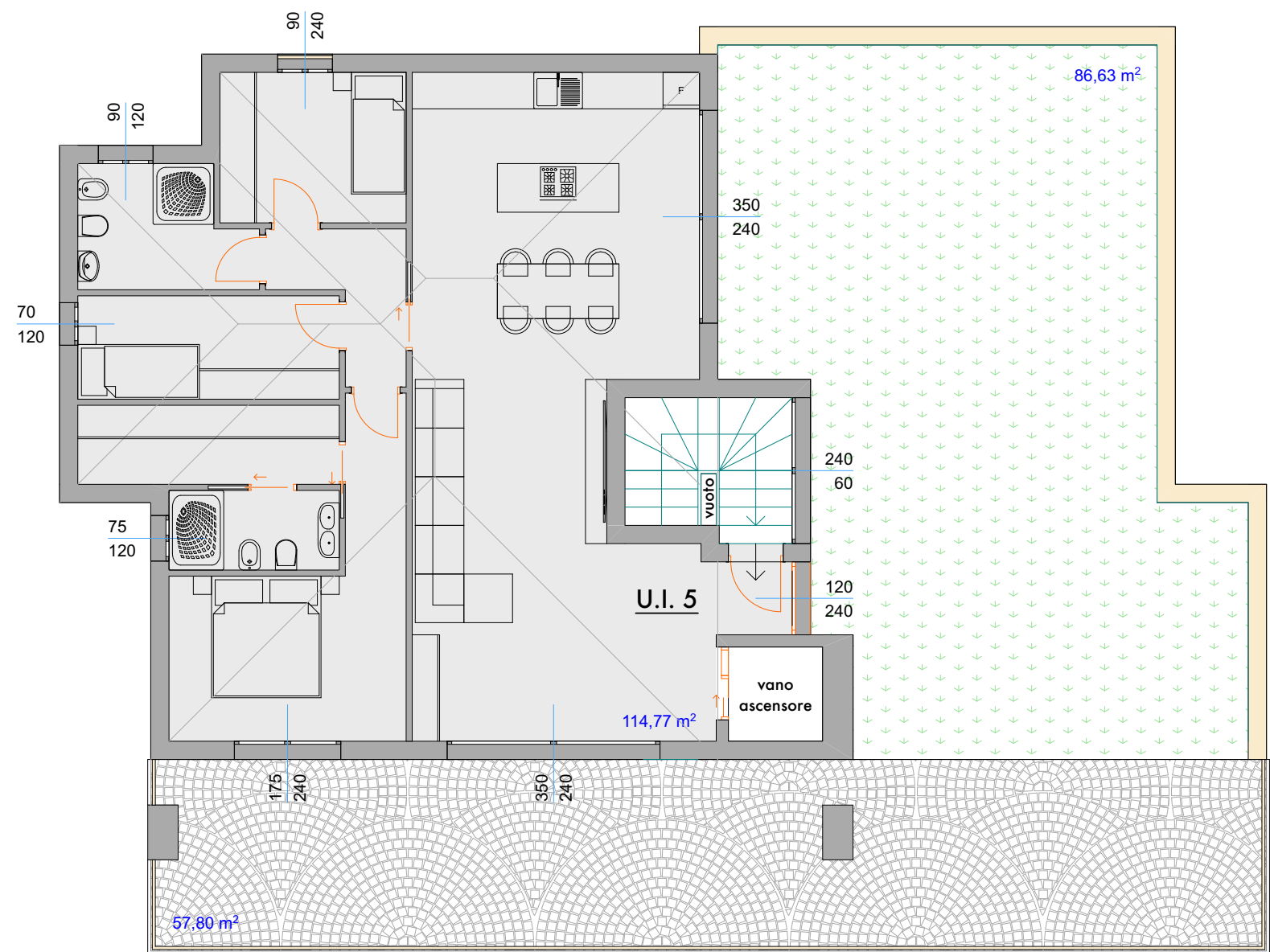
PIANO MANSARDA
